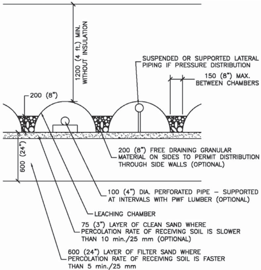
LEACHING CHAMBERS IN AN ABSORPTION BED
